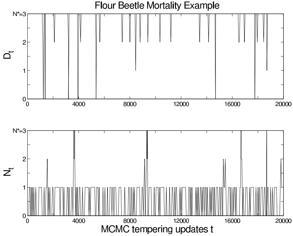
Figure 4: Flour Beetle Mortality example of Section 3.2. Forward simulation of the dominating process D_t (upper graph) with tempering process Z_t = (X_t, N_t) , (N_t , lower graph) for geometric average pseudo-prior, \bar{\pi} = \sqrt{\pi_N \pi_D} . Notice that D_t \geq N_t at each MCMC update. At top tempering level N^* = 3 , the tempering distribution coincides with that of the target distribution G .
