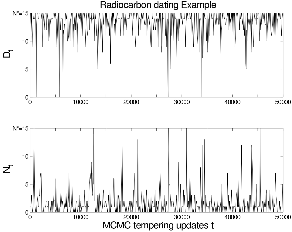
Figure 6: Radiocarbon dating example, Section 3.3. Forward simulation of the dominating process D_t (upper graph) with tempering process Z_t = (X_t, N_t) ( N_t , lower graph) for geometric average pseudo-prior, \bar{\pi} = \sqrt{\pi_N \pi_D} . At top tempering level N^* = 15 , the distribution has the full set of variables of the target distribution, whilst distributions at lower tempering levels have some subset of the full variable set.
