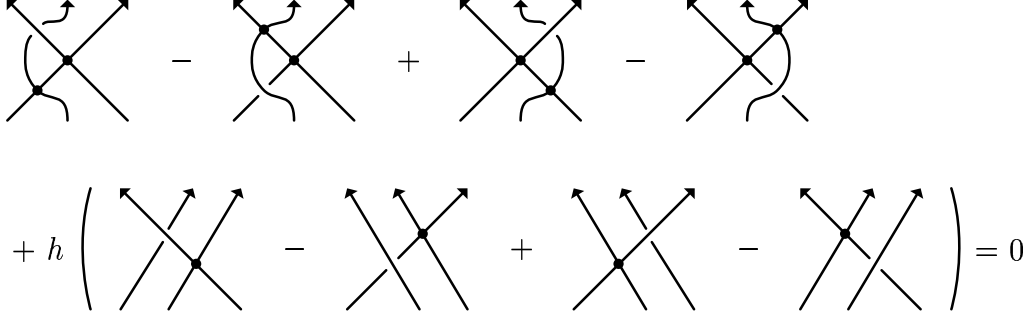
FIGURE 5. The 8T-relation.
