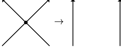
FIGURE 12. The smoothing of a chord.
