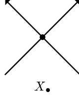
FIGURE 2. A double point X_\bullet .
