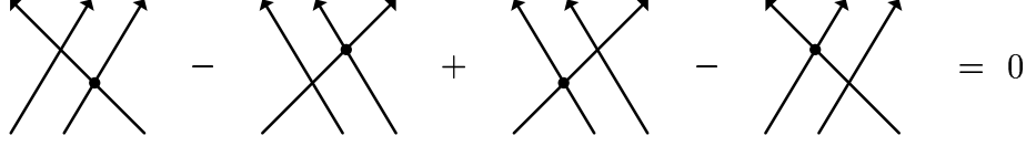
FIGURE 11. The 4TS-relation.
