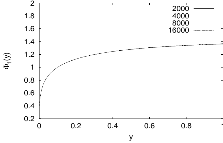
Figure 2: Finite size scaling of the average distance travelled by the random walker for the Ising model.
