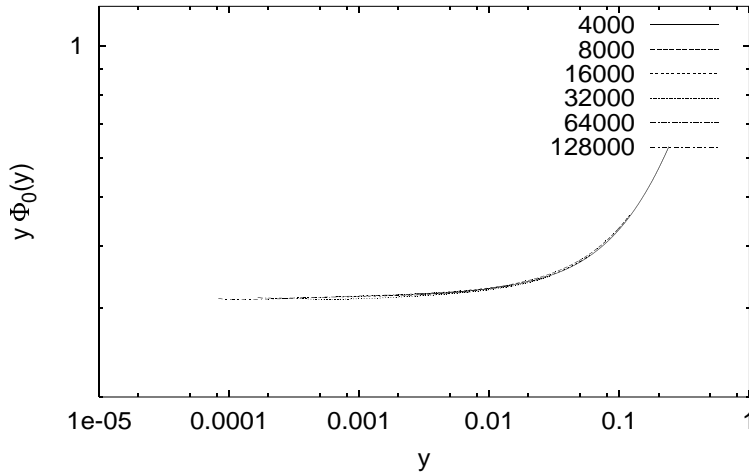
Figure 3: Small time behaviour of the return probability for the c = -2 model.
