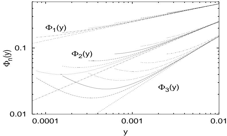
Figure 4: Small time behaviour of the moments \Phi_n(y) for the c = -2 model. N = 4 –128K from right to left for each distribution. The straight lines are \propto y^{nd_s/2d_h} for d_s = 2 and d_h = 3.58 . Slow convergence is observed as N \rightarrow \infty .
